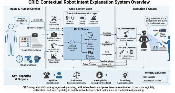
Fig. 1. CRIE system overview. The CRIE Planner receives task goals, workspace observations, action chunk feedback, and entropy-based uncertainty, and produces structured commands, intent explanations, and role assignments via a learned grounding head. A proactive communication layer delivers intent through speech and visual overlay. (AI-assisted figure, reviewed by authors.)
